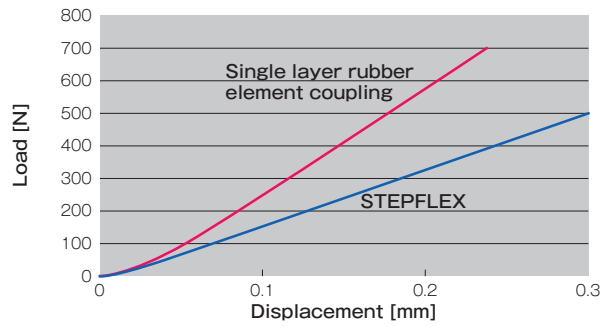
Comparison of counterforces along the axial direction
